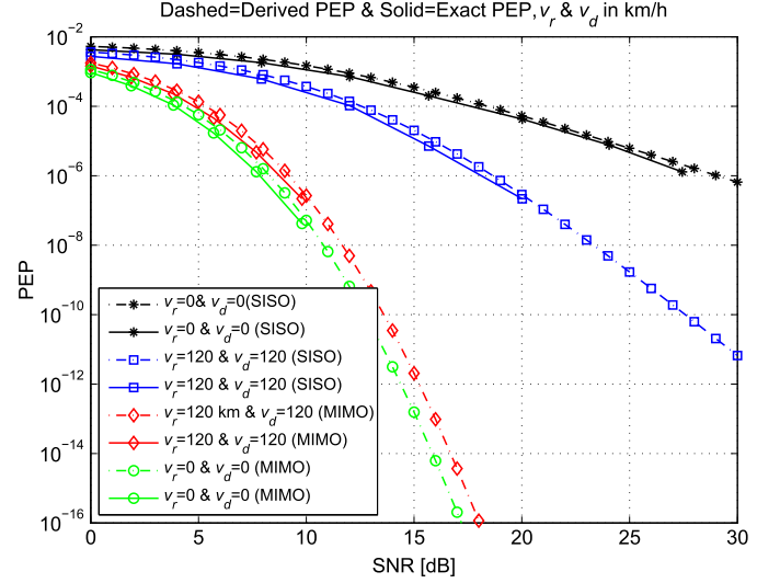
Fig. 3. Comparison of the derived PEP in (19) and the exact PEP for the MIMO scheme.
