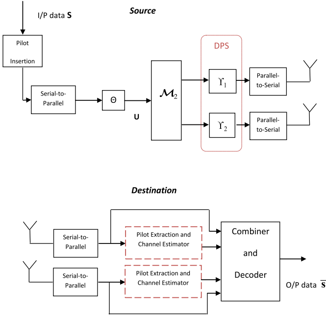
Fig. 2. Alamouti-code based MIMO cooperative transmission scheme.
