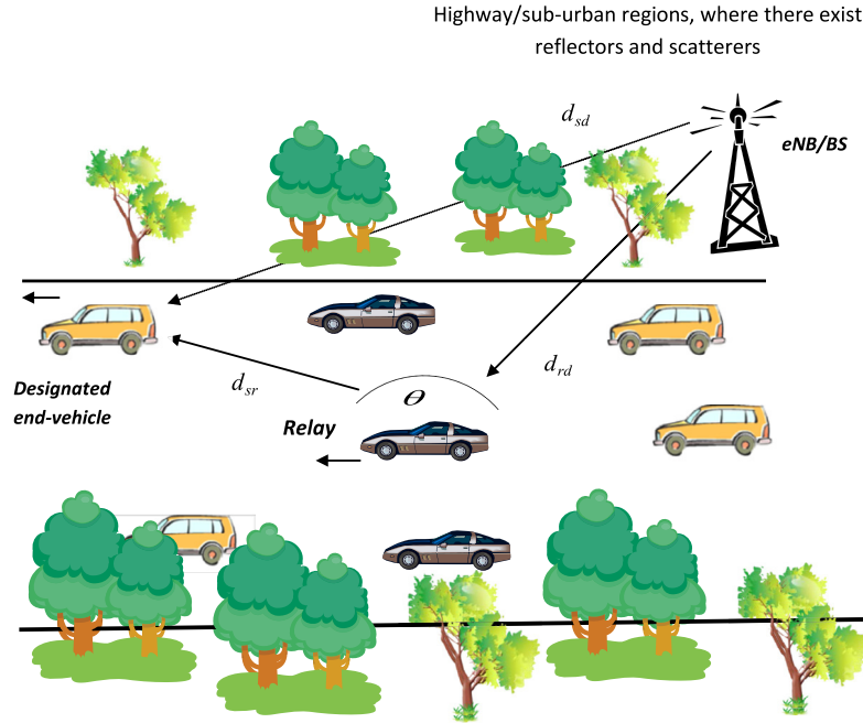
Fig. 1. Cooperative best-relay selection model in a highway/suburban area with 2 \times 2 MIMO deployment.
