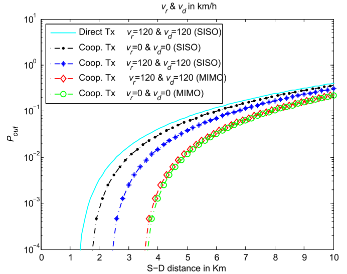
Fig. 5. S \rightarrow D distance in km versus outage probability.
