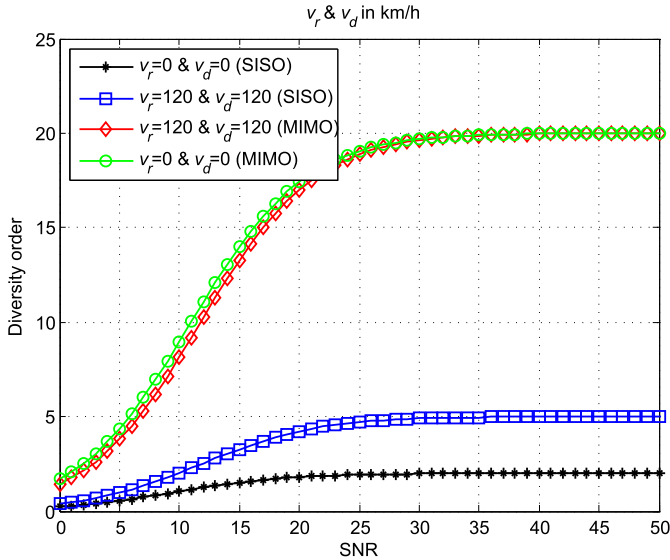
Fig. 4. Diversity order of the MIMO cooperative relaying scheme for an LTE-A downlink session.
