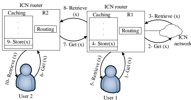
Fig. 11. Random requests attack (normal case): 1- User1 requests for ICN content named (x). 2- R1 router tries to find the content (x). 3- R1 retrieves the content from ICN network. 4- R1 caches the content (x). 5- User1 retrieves the content (x). 6- User2 requests the same content (x) via R2 router. 7- R2 tries to find the closest copy, which exists in R1 router. 8- R1 sends the content to R2 router. 9- R2 caches the content (x). 10- User2 retrieves the content (x).
