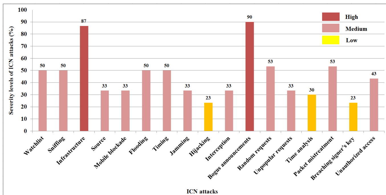
Fig. 14. Severity levels of ICN attacks
