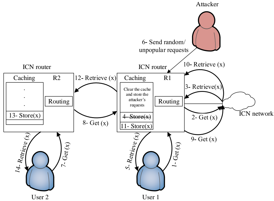
Fig. 12. Random requests attack (attacked case): 1- User1 requests for ICN content named (x). 2- R1 router tries to find the content (x). 3- R1 retrieves the content from ICN network. 4- R1 caches the content (x). 5- User1 retrieves the content (x). 6- An attacker sends a large number of random/unpopular requests to violate the cache. 7- User2 requests the same content (x) via R2 router. 8- R2 tries to find the closest copy and sends request to R1. 9- R1 router tries to find the content (x). 10- R1 retrieves the content from ICN network. 11- R1 caches the content (x). 12- R1 sends the content to R2. 13- R2 caches the content (x). 14- User2 retrieves the content (x).
