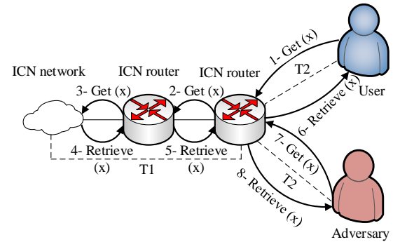
Fig. 9. Time analysis attack: 1- A user requests for ICN content named (x). 2 and 3- ICN routers try to find the content (x). 4 and 5- ICN routers forward the content (x) to the requested user. 6- The user retrieves the content (x) in total time T_1+T_2 . 7- An adversary requests for the content (x). 8- The adversary retrieves the content (x) in time T_2 only, as routers cache the content.
