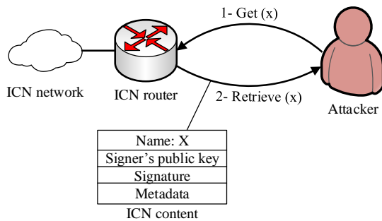
Fig. 13. Breaching signer's key attack: 1- An attacker requests for ICN content named (x). 2- The attacker retrieves the content (x) that contains signer's public key and signature, which can be used with the content itself to determine the signer's key.
