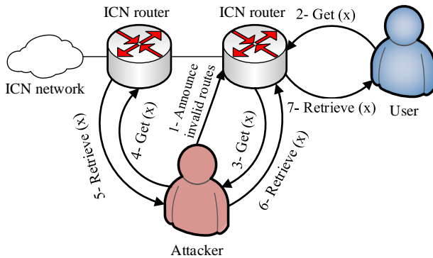
Fig. 8. Interception attack: 1- An attacker announces invalid routes for some content including (x). 2- A user requests for ICN content named (x). 3- ICN router redirects the user request to the attacker's malicious routes. 4- The attacker forwards the request to get the actual content. 5- The attacker retrieves the content (x). 6- The attacker forwards the content to the requested user. 7- The user retrieves the content (x).
