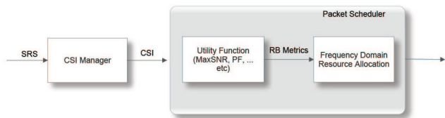
Figure 2: Scheduler Workflow.
