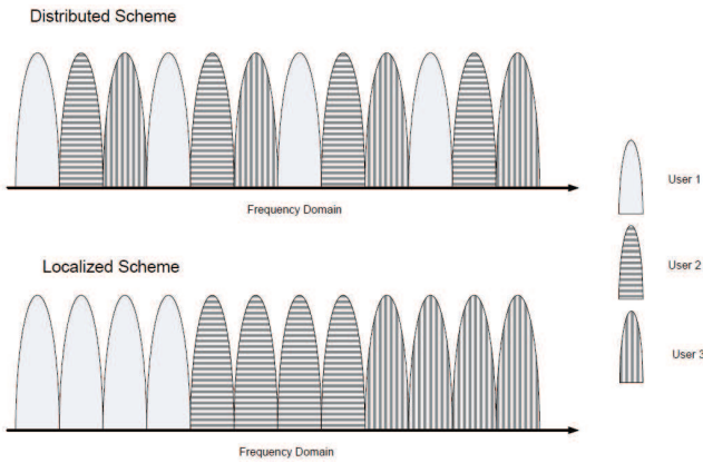
Figure 1: Distributed vs. Localized FDMA allocation schemes.
